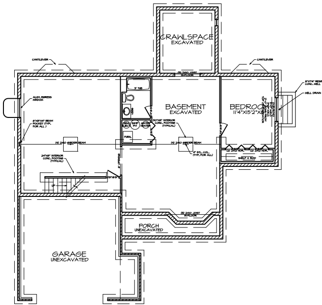
1 FOUNDATION PLAN A-2
